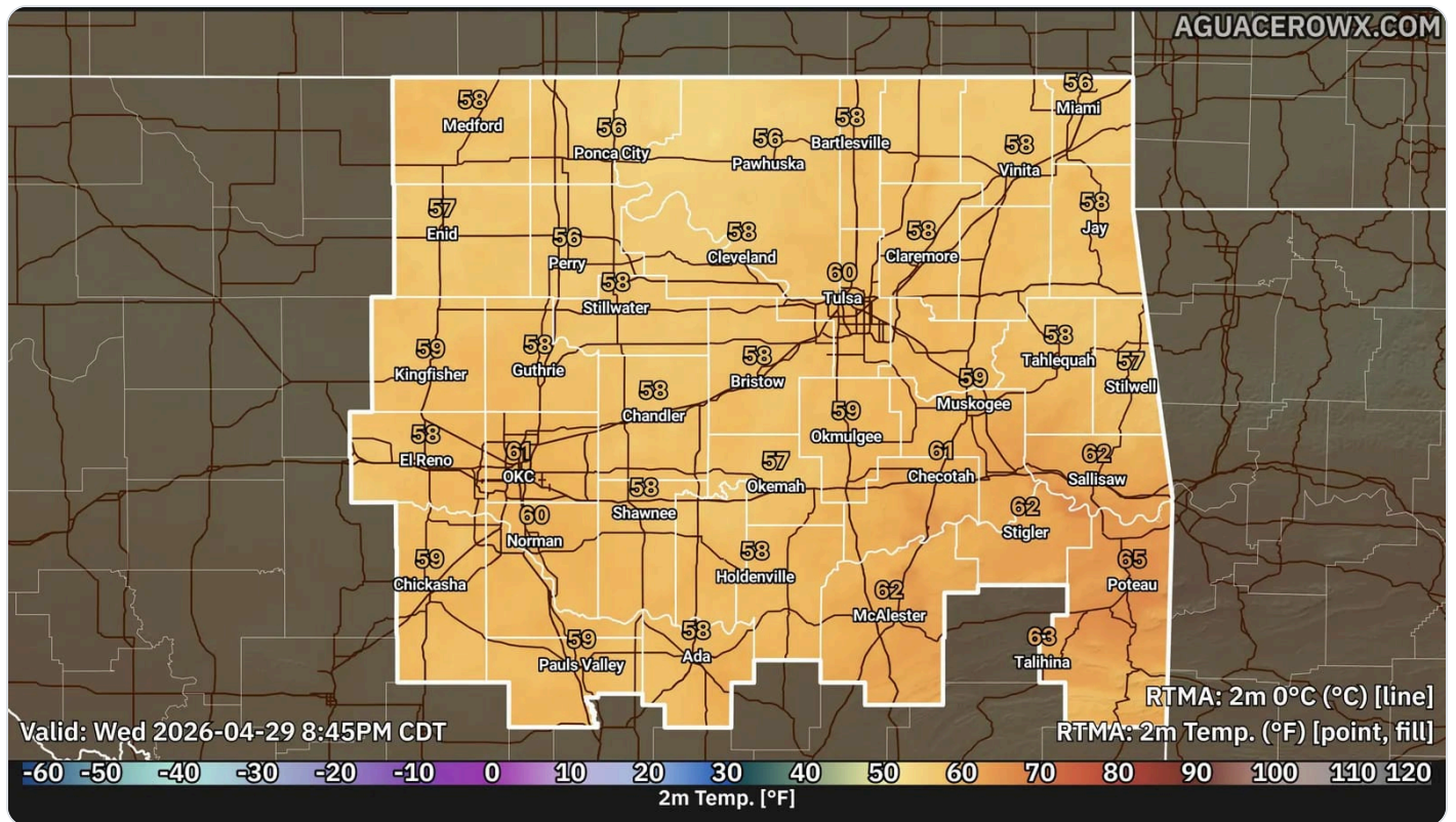
RTMA 2 m temperature with Oklahoma highlighted and county values plotted.
