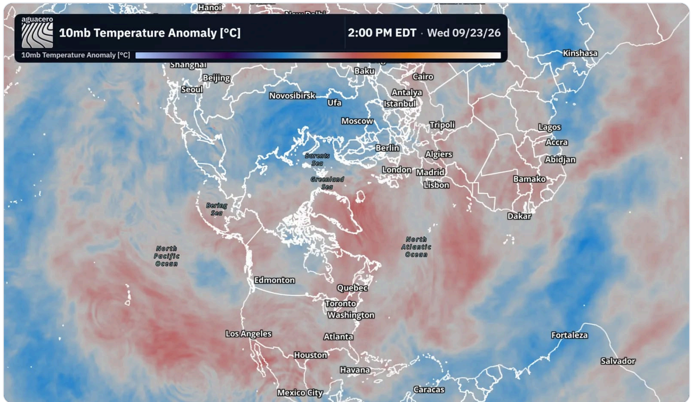
10 mb temperature anomaly on a polar stereographic projection.
