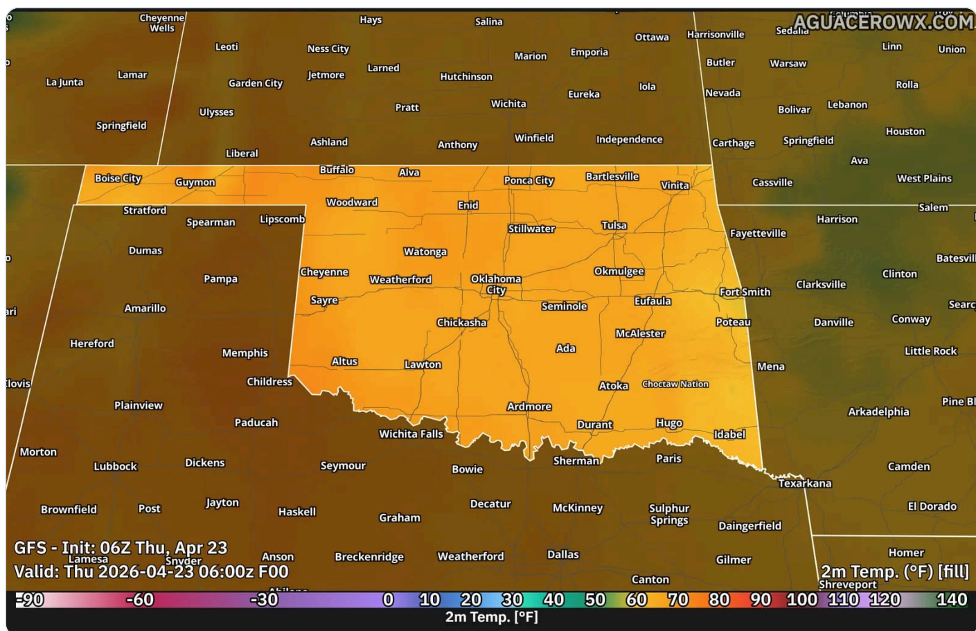
GFS 2 m temperature with a custom Oklahoma layer.
