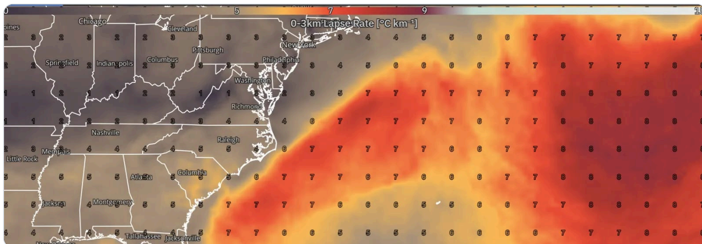
0–3 km lapse rates with grid point values.
