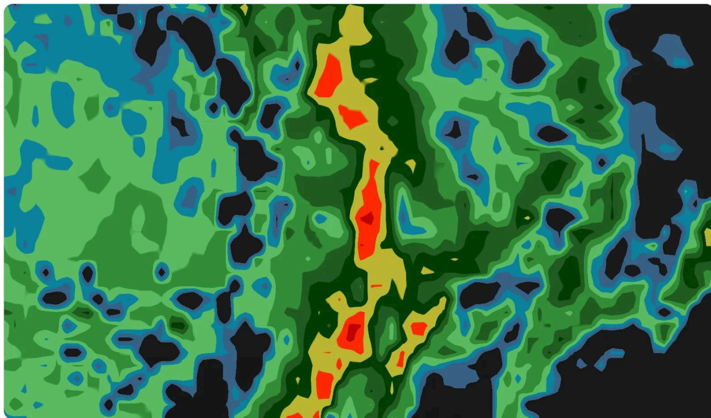
A hard-step colormap on a model precipitation field.
