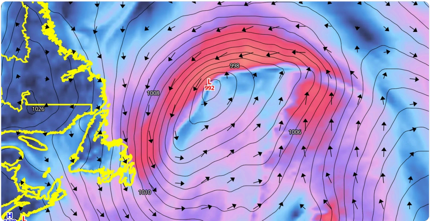
Wind vectors around a North Atlantic low.
